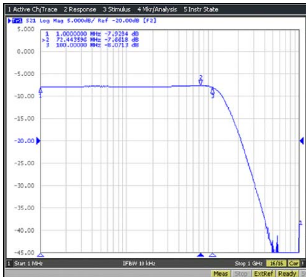
FIGURE 13. AMPLIFIER FREQUENCY RESPONSE AT 200MSPS
