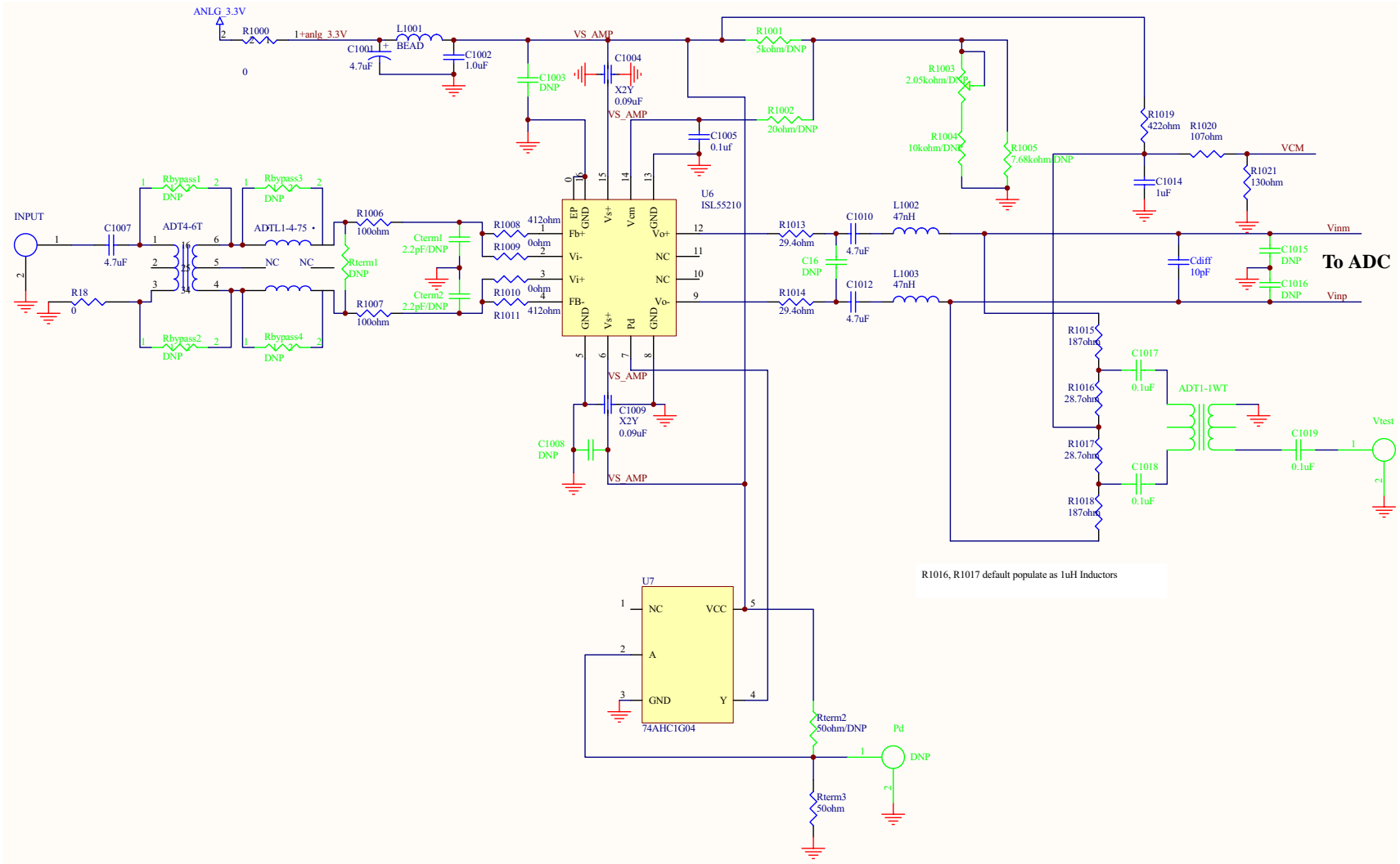
FIGURE 39. ISLA112P50/55210EV1Z (2 OF 3)
