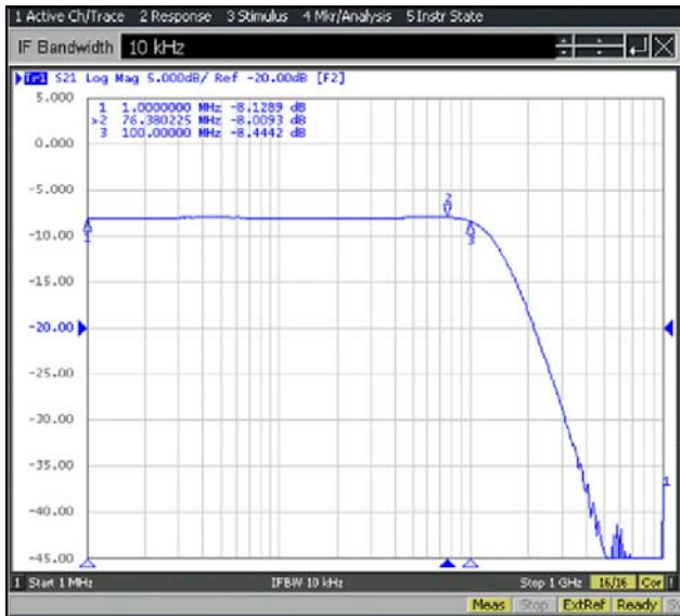
FIGURE 12. AMPLIFIER FREQUENCY RESPONSE AT 500MSPS
