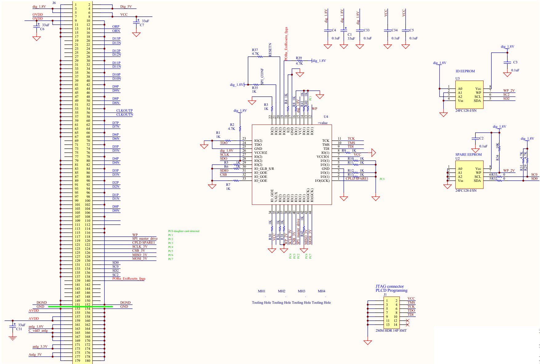
FIGURE 40. ISLA112P50/55210EV1Z (3 OF 3)
