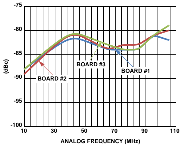
FIGURE 24. HD3 at 450MSPS
