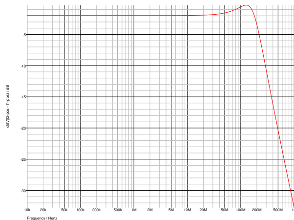
FIGURE 11. SIMULATED DIFFERENTIAL FILTER RESPONSE
